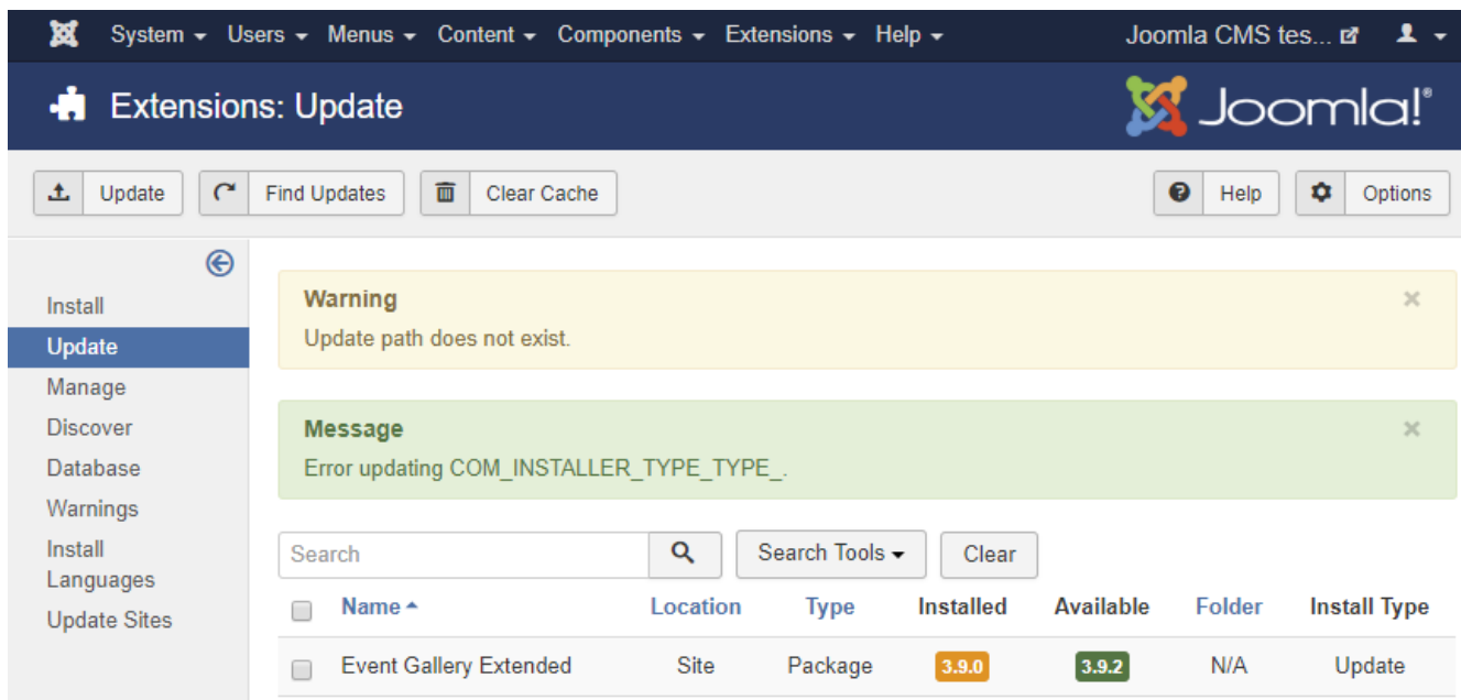
Figure 78. Update fails
