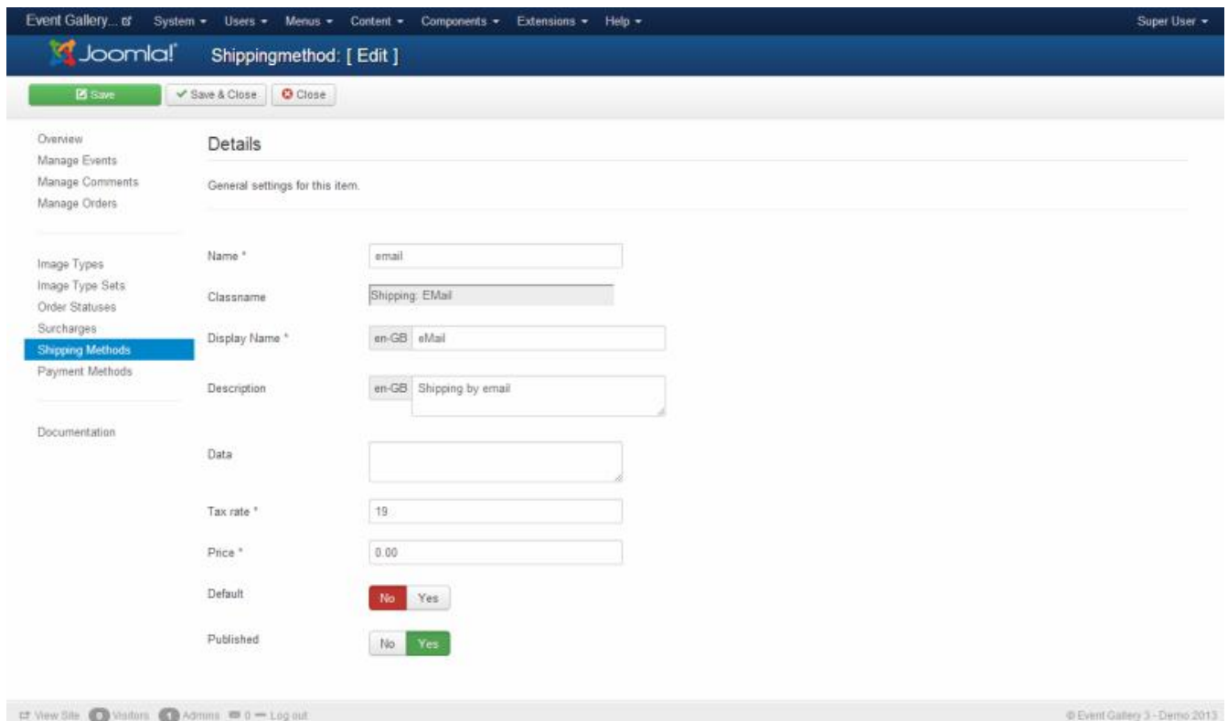
Figure 62. Shipping Method
