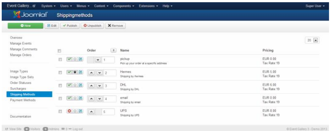
Figure 61. Shipping Methods
