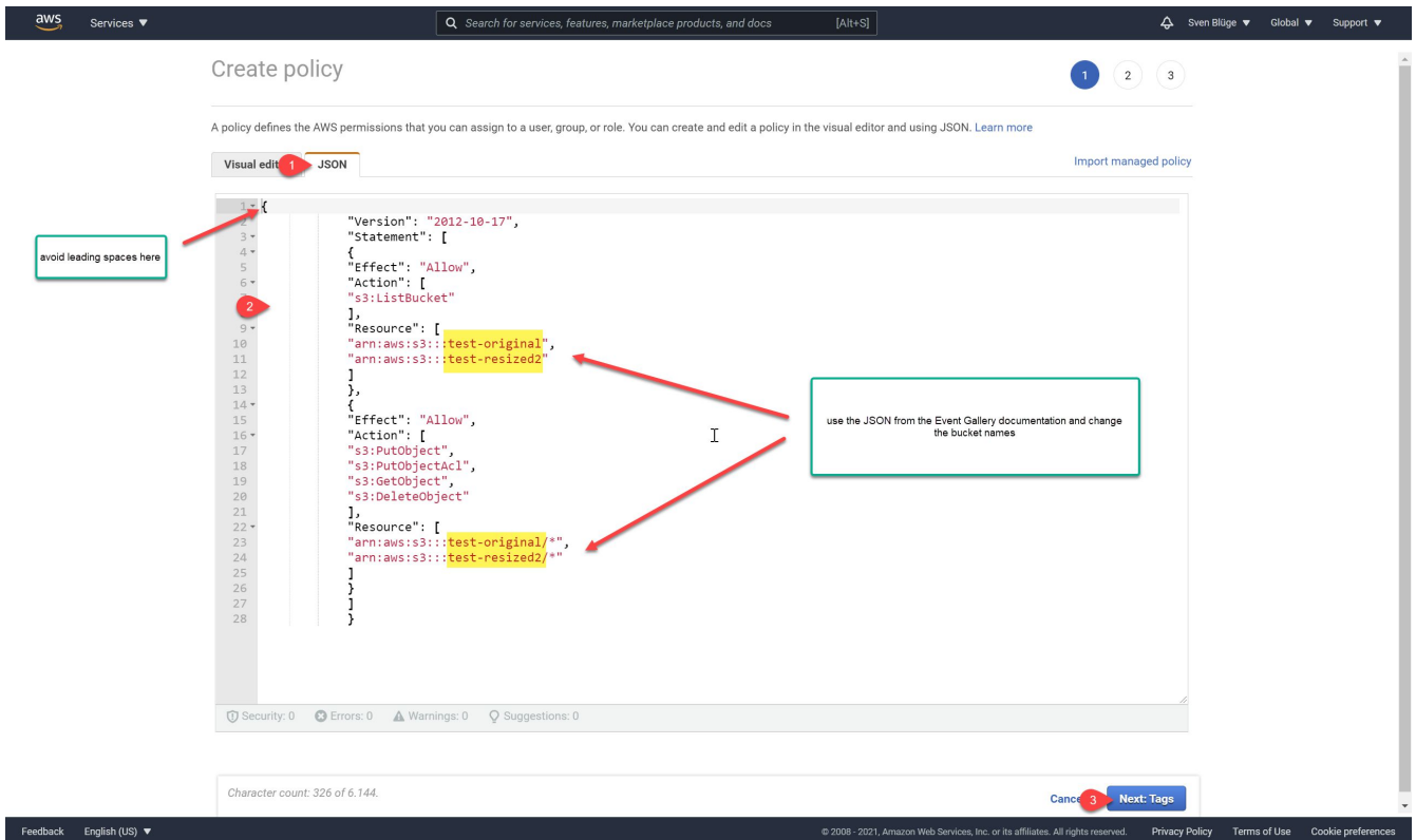
Figure 32. Copy and modify the access policy JSON from above
