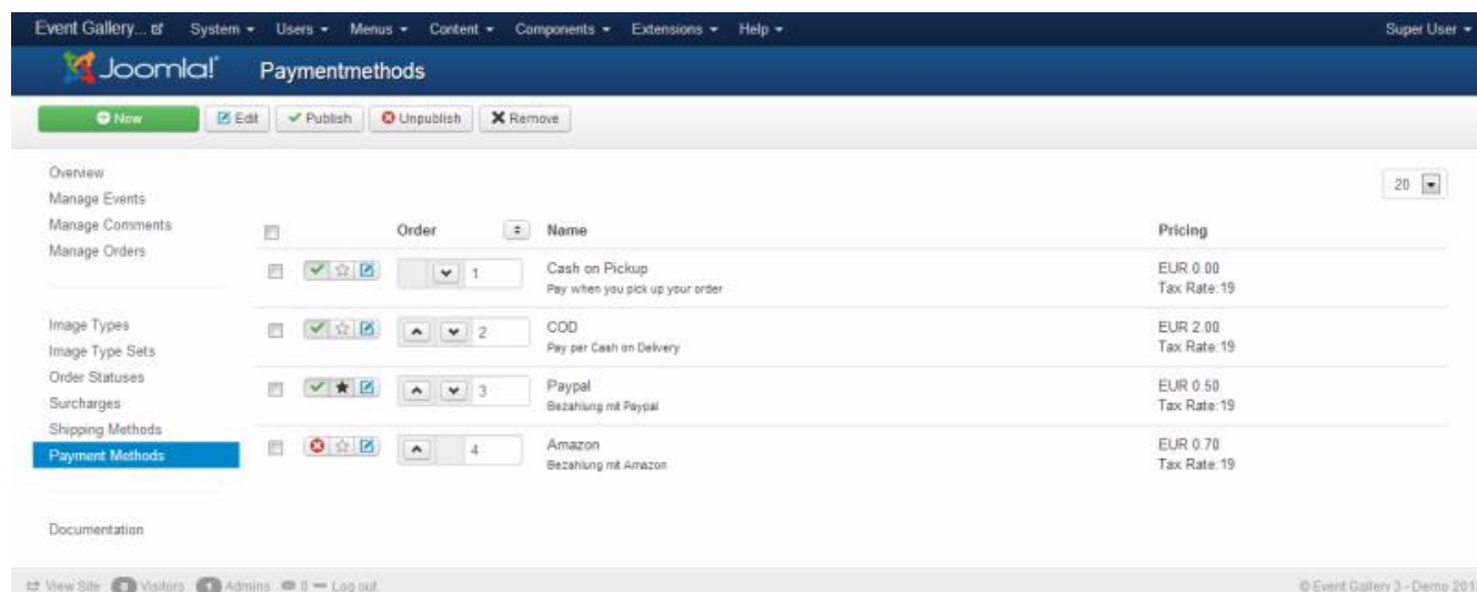
Figure 55. Payment Methods
