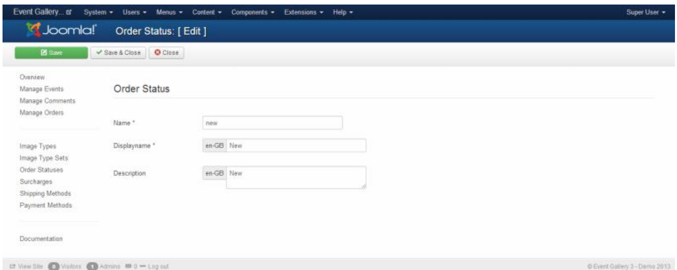
Figure 50. Order Status
