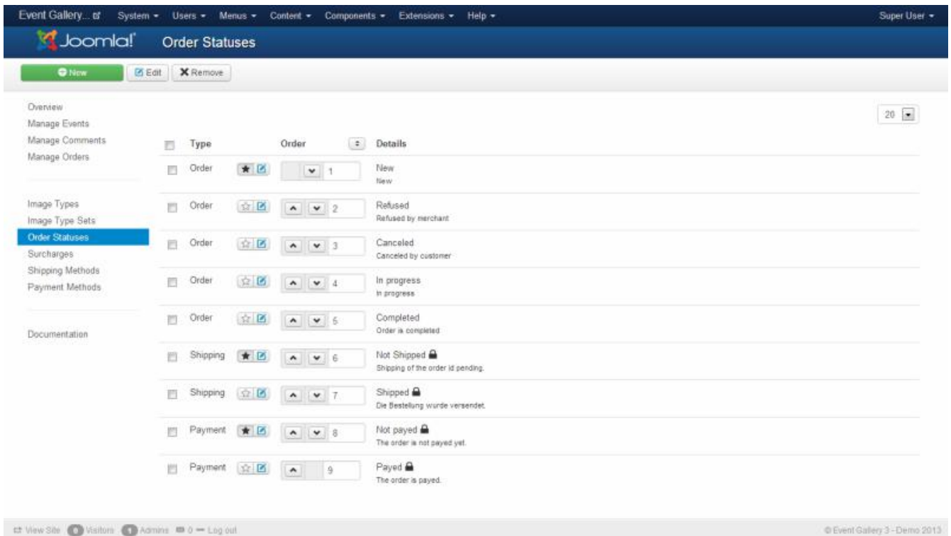
Figure 49. Order Statuses
