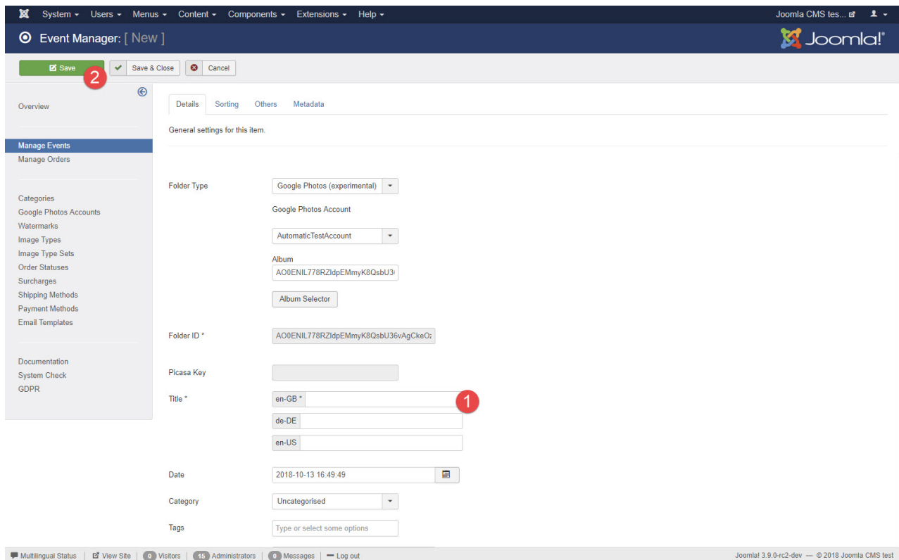
Figure 44. Select Album
