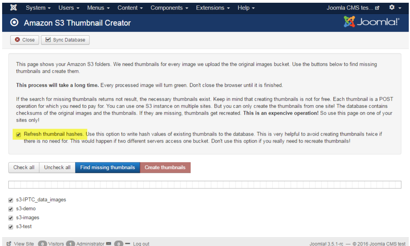
Figure 22. Thumbnail Creator
