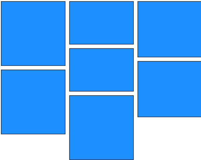
Tile Layout
