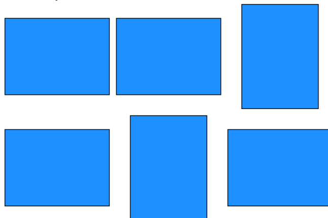
Grid Layout
