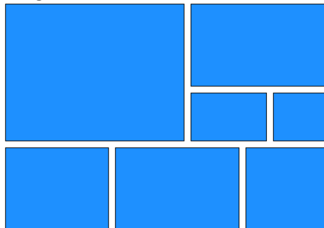
Image List
