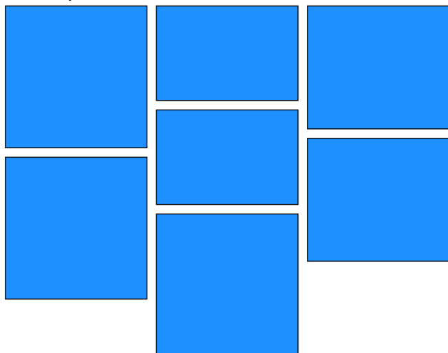
Tile Layout
