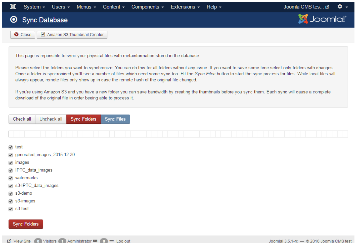
Figure 4. Sync Database
