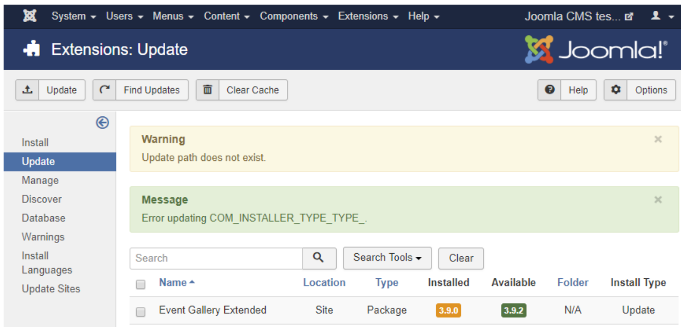
Figure 78. Update fails
