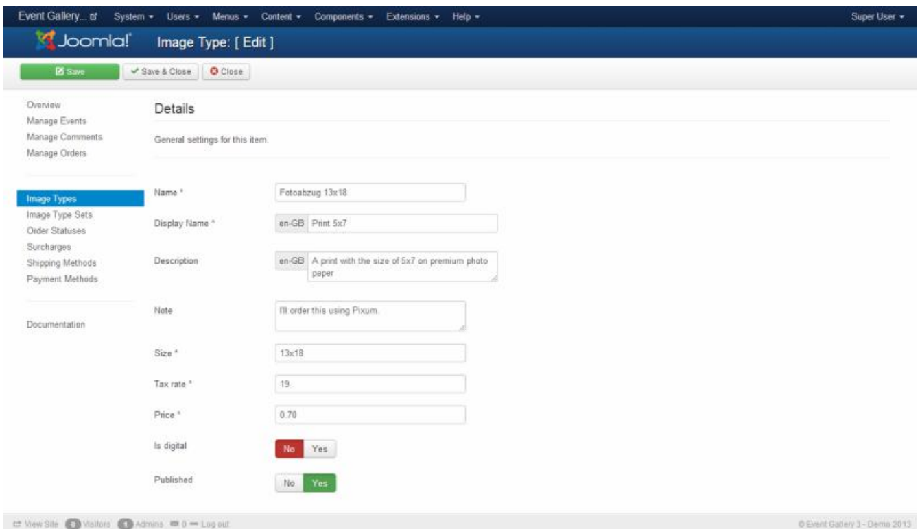
Figure 52. Image Type
