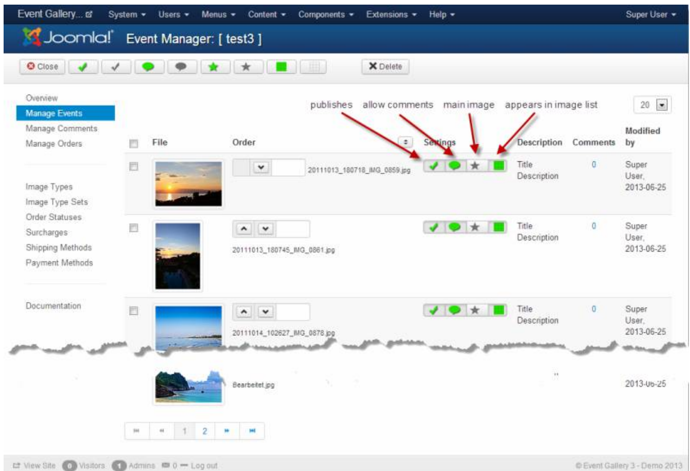
Figure 12. Event Page
