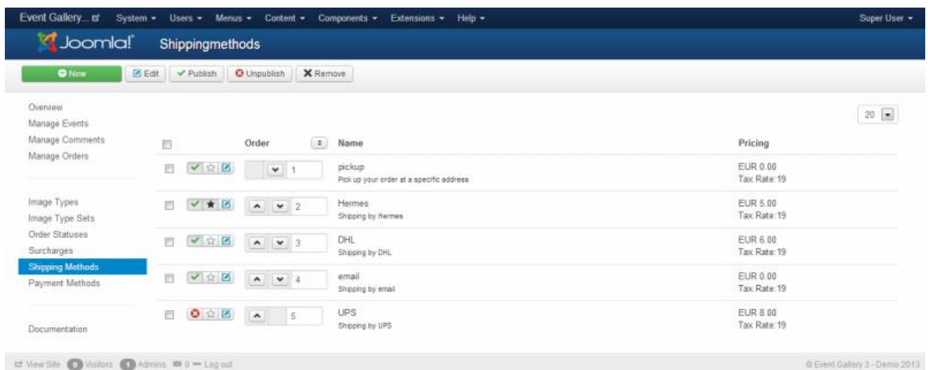
Figure 61. Shipping Methods
