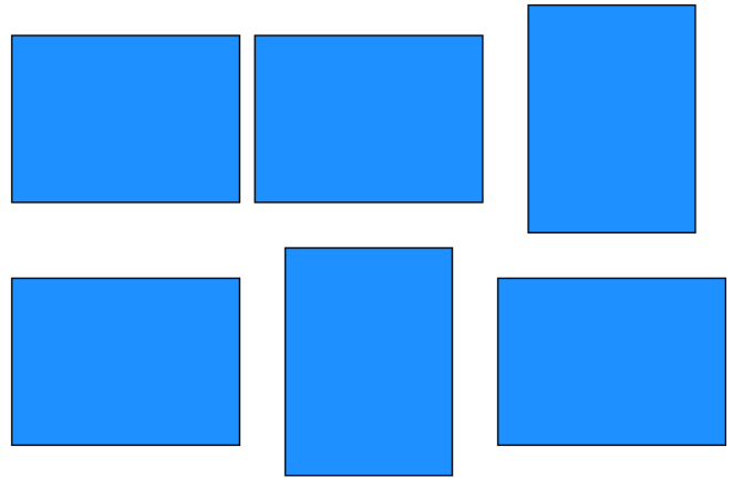
Grid Layout
