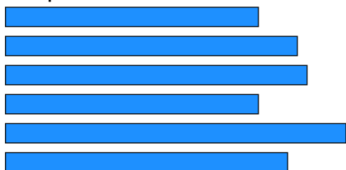
Simple List
