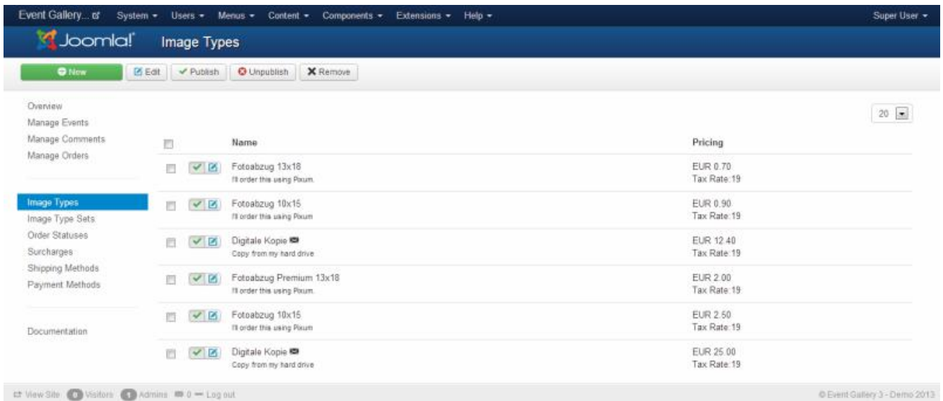
Figure 51. Image Types
