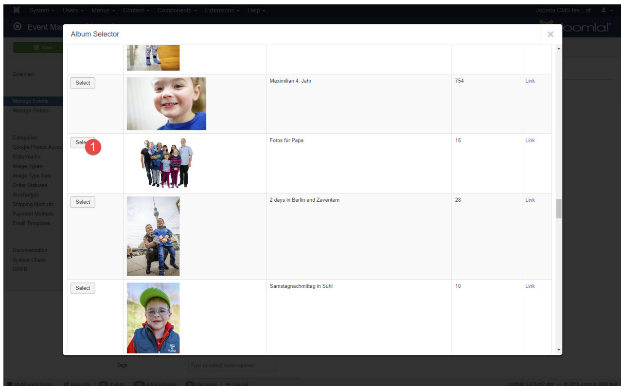
Figure 43. Select Album
