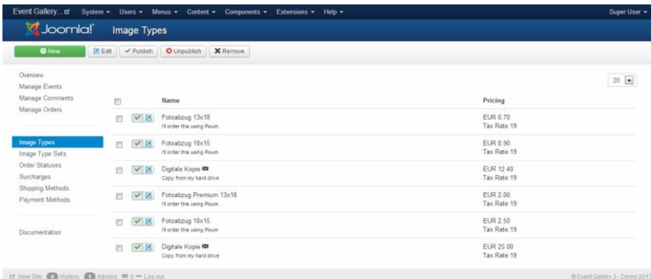
Figure 45. Image Types
