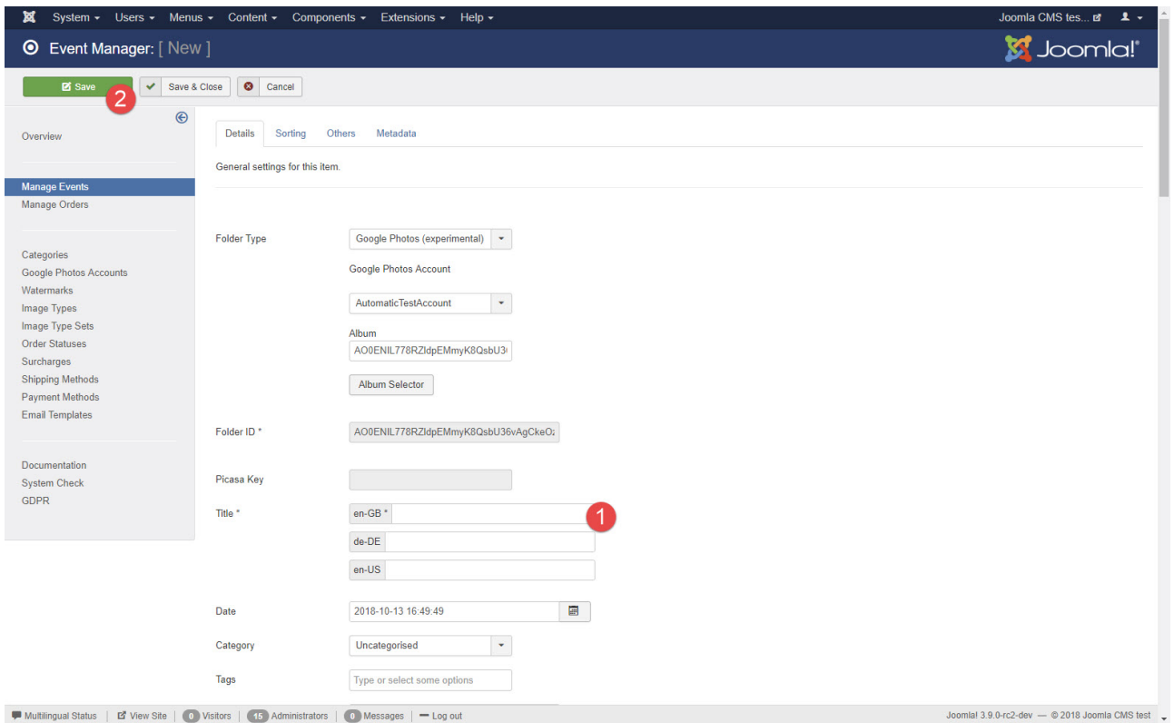
Figure 38. Select Album
