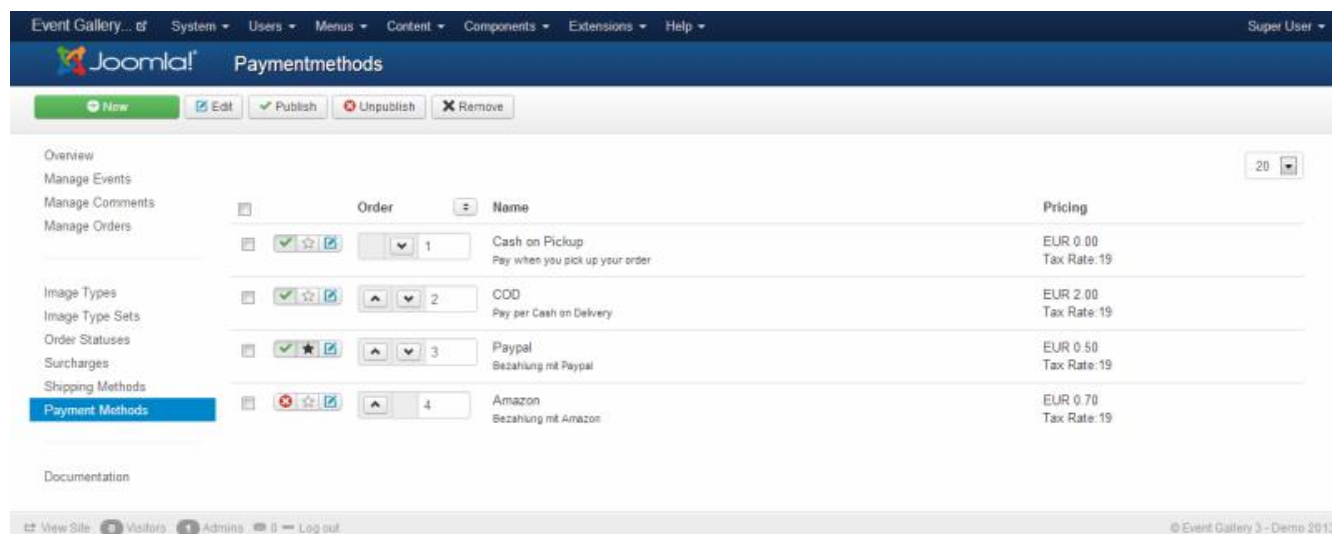
Figure 49. Payment Methods
