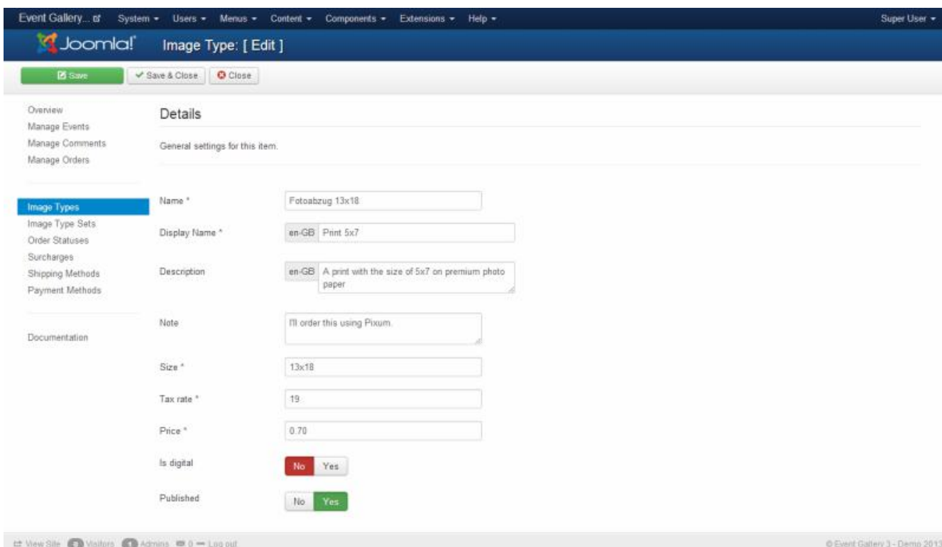
Figure 46. Image Type
